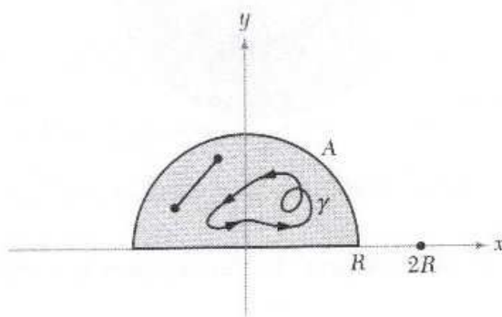
Figure 2.3.16: Convex region.
