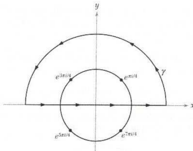
Figure 4.2.7: The curve \gamma in Example 4.2.5.
