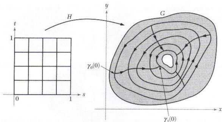
Figure 2.3.13: Closed-curve homotopy.
