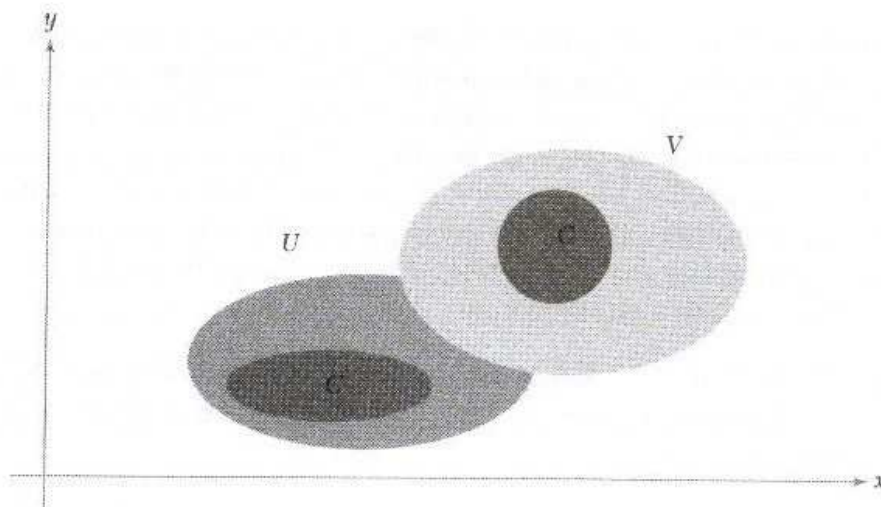
Figure 1.4.4: The set C is not connected.
