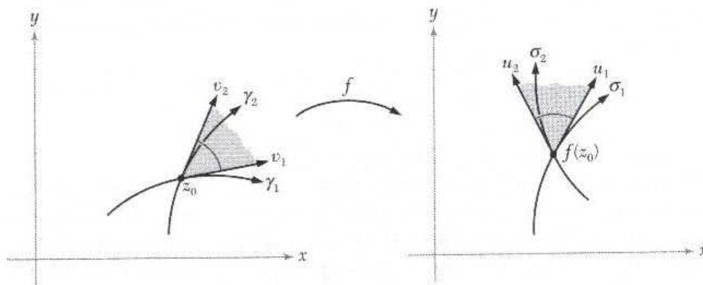
Figure 1.5.2: Preservation of angles by a conformal map.
