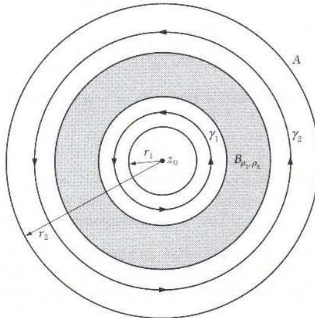
Figure 3.3.2: Construction of the curves \gamma_1 and \gamma_2 .
