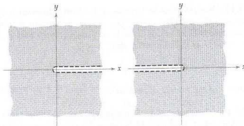
Figure 1.5.3: Two regions of validity of polar coordinates.
