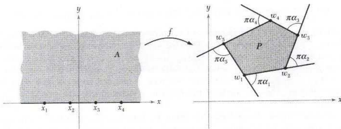
Figure 5.2.6: Schwarz-Christoffel Formula.
