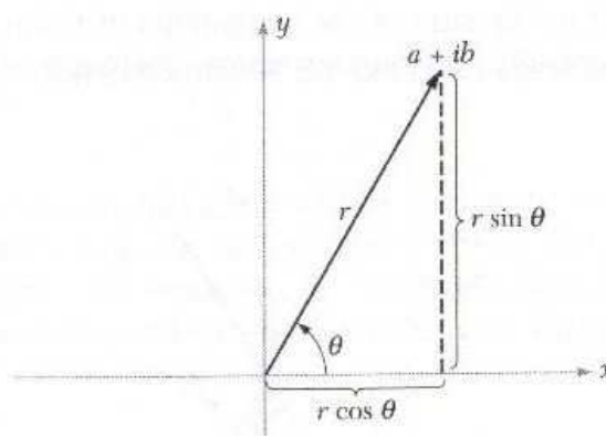
Figure 1.2.3: Polar coordinate representation of complex numbers.
