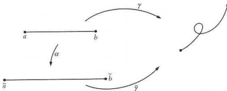
Figure 2.1.4: Reparametrization.
