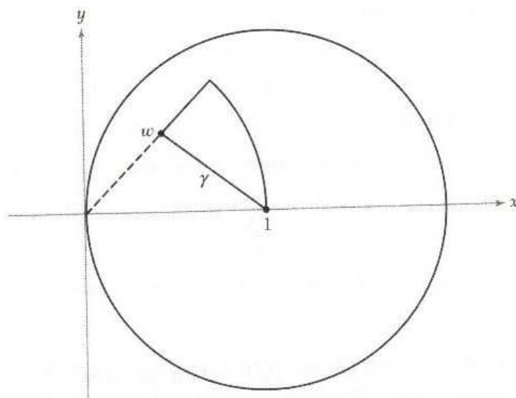
Figure 3.1.9: Path for computing \log w on D(1; 1) .
