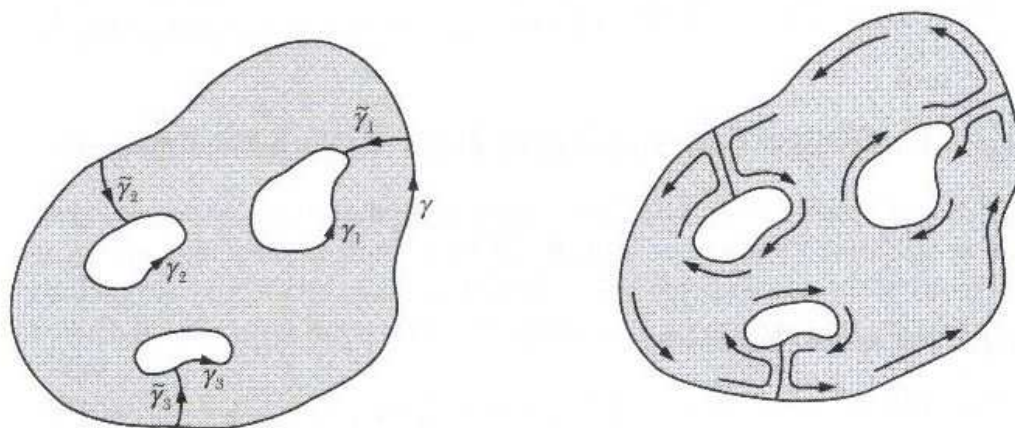
Figure 2.2.10: Path used to prove the Generalized Deformation Theorem.
