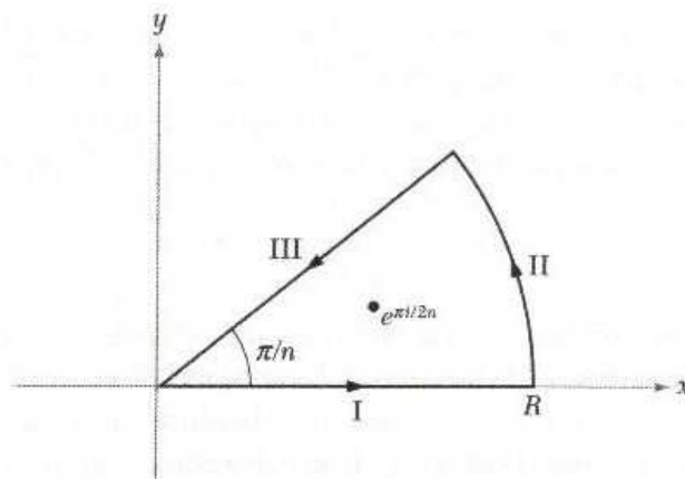
Figure 4.3.7: Contour for Worked Example 4.3.20.
