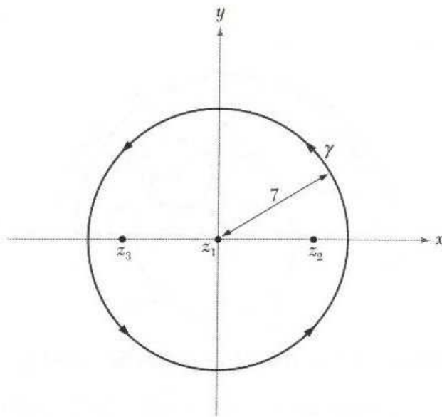
Figure 4.2.9: The curve \gamma contains three singularities.
