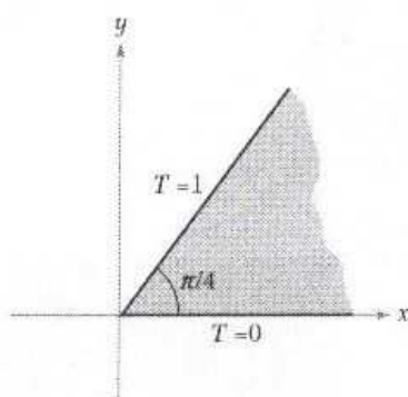
Figure 5.3.18: Find the temperature for these regions (Exercises 1 and 2).
