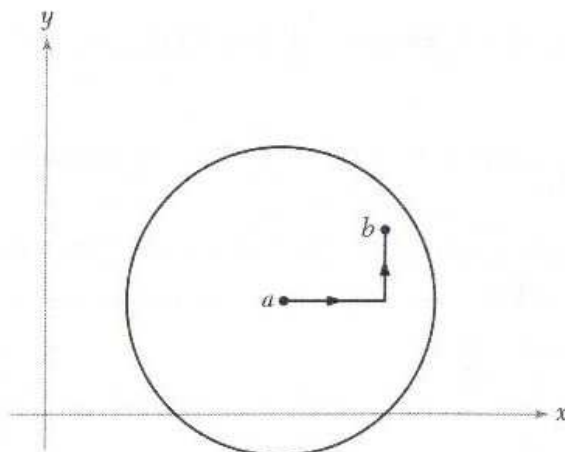
Figure 2.3.3: The path \langle\langle a, b \rangle\rangle .
