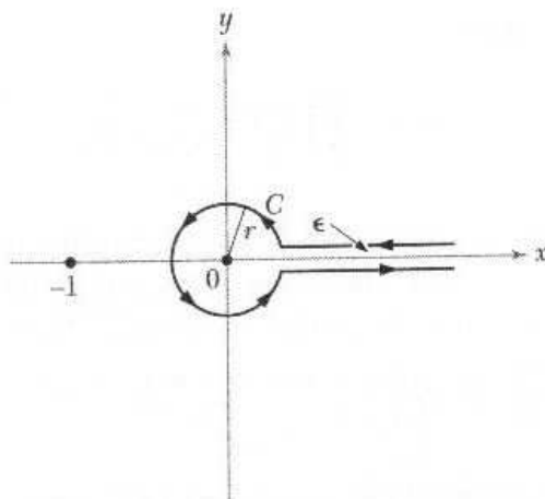
Figure 7.1.2: Contour for Hankel's formula.
