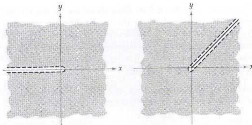
Figure 1.6.3: Regions of analyticity for z \mapsto z^a .
