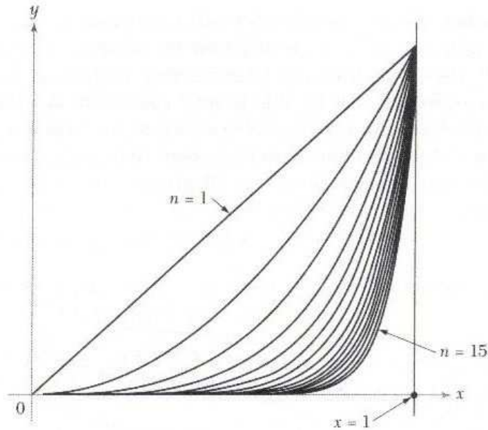
Figure 3.1.2: Convergence of x^n to 0 is not uniform on \{x \mid 0 \leq x < 1\} .
