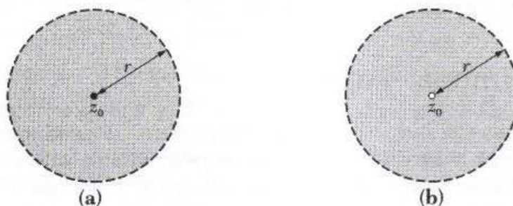
Figure 1.4.1: Open set.
