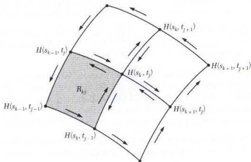
Figure 2.3.15: Cancellation of edges of the subsquares in the proof of the deformation theorems.
