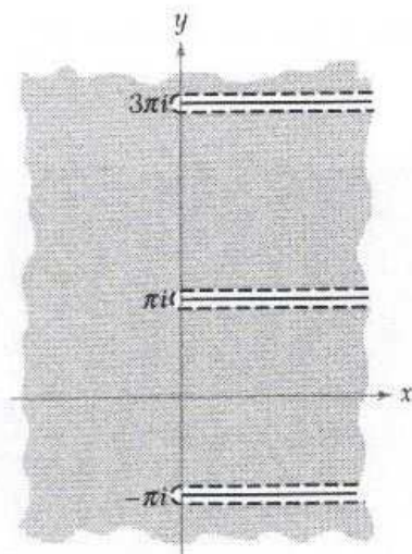
Figure 1.6.4: Region of analyticity of \sqrt{e^z + 1} .
