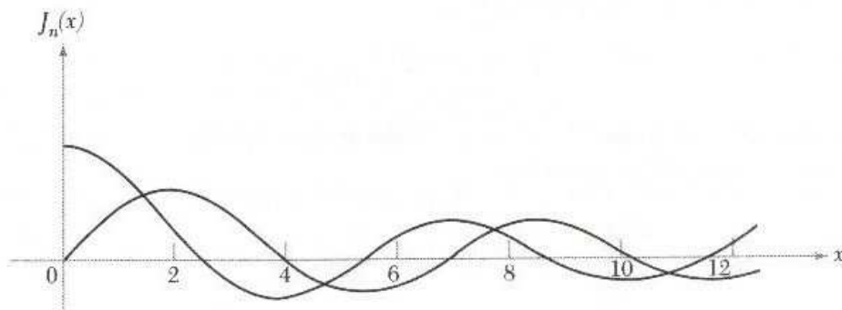
Figure 7.3.3: Bessel functions J_0(x) , J_1(x) .
