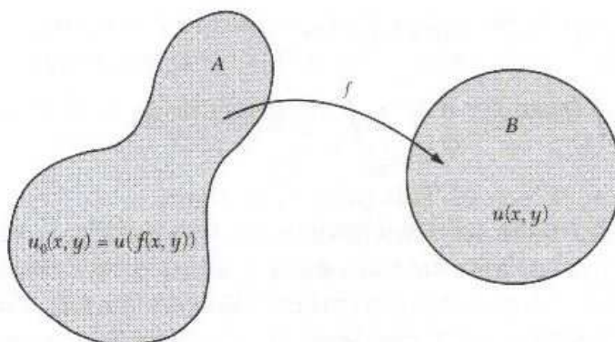
Figure 5.3.2: Transformation of harmonic functions.
