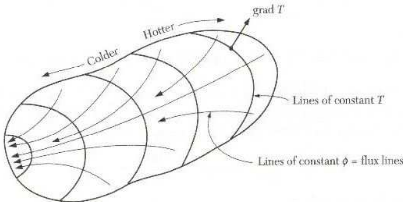
Figure 5.3.4: Heat conduction.
