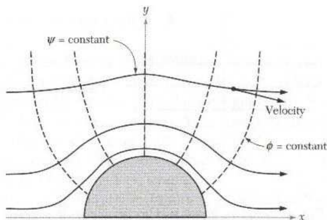
Figure 5.3.17: Streamlines for flow around a cylinder.
