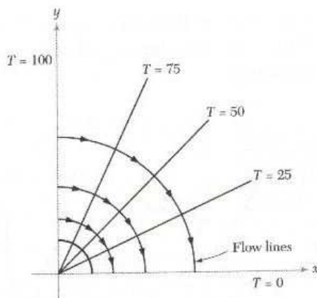
Figure 5.3.6: Isotherms and flux lines for Example 5.3.1.
