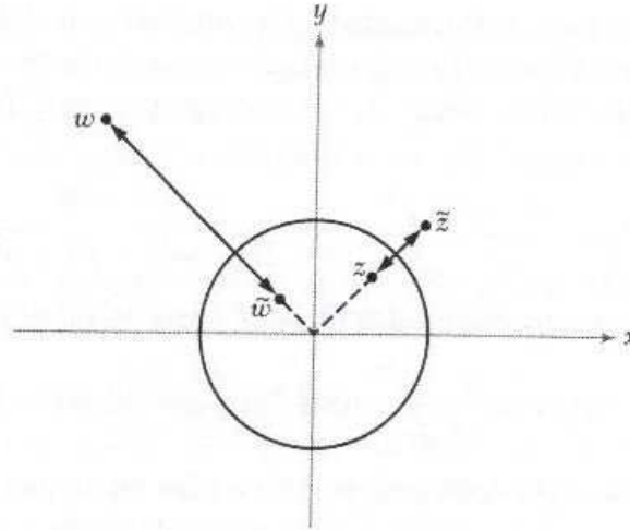
Figure 2.5.3: Reflection of a complex number in a circle.
