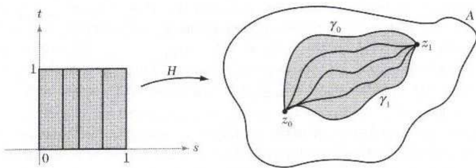
Figure 6.1.11: Homotopy between \gamma_0 and \gamma_1 .
