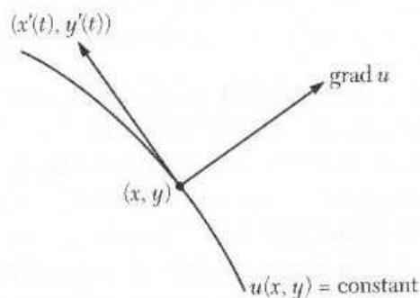
Figure 1.5.4: Harmonic conjugates: u = x^2 - y^2 , v = 2xy , f(z) = z^2 .
