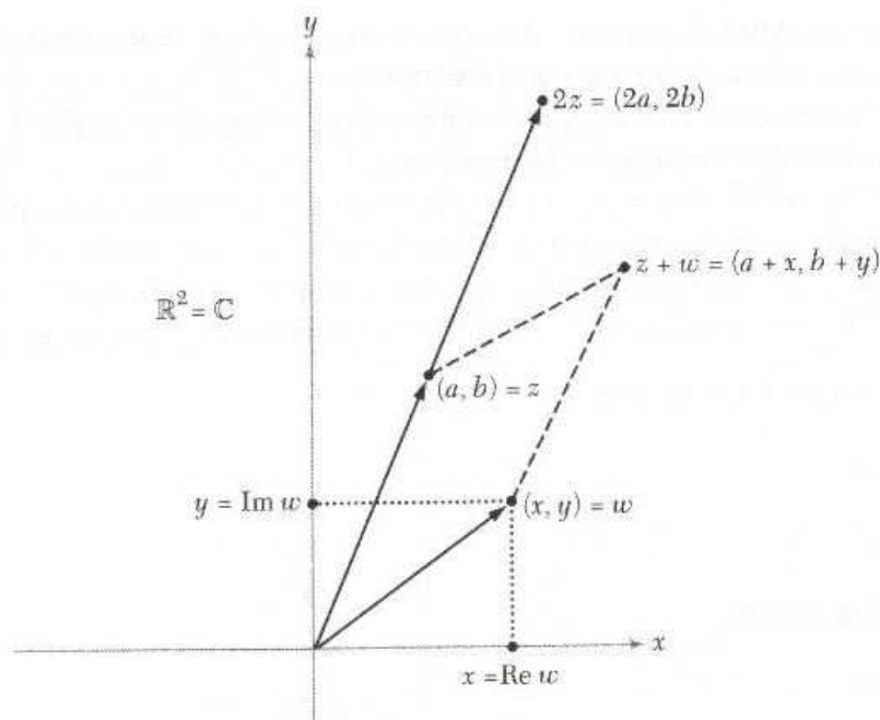
Figure 1.1.1: The geometry of complex numbers.
