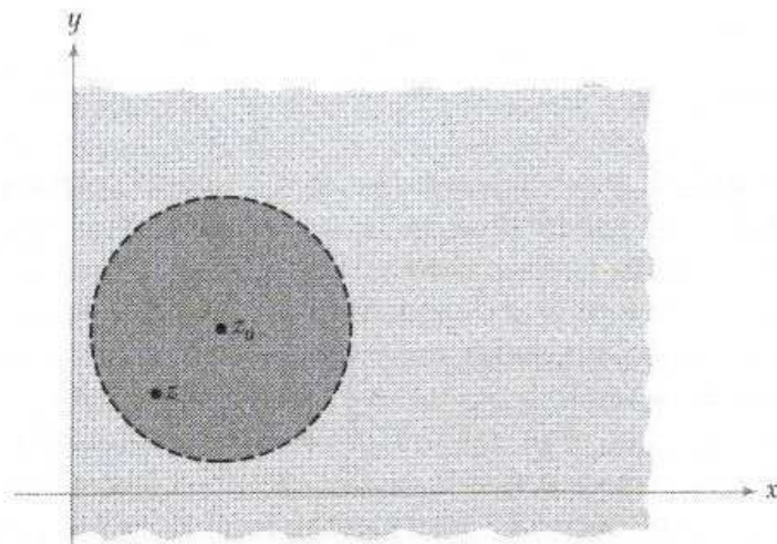
Figure 1.4.9: Open right half-plane.
