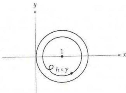
Figure 6.2.3: The image of \gamma under h .
