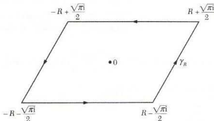
Figure 4.3.12: The contour used for \int_{-\infty}^{\infty} e^{-x^2} dx .
