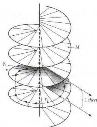
Figure 6.1.14: Riemann surface for \log z .
