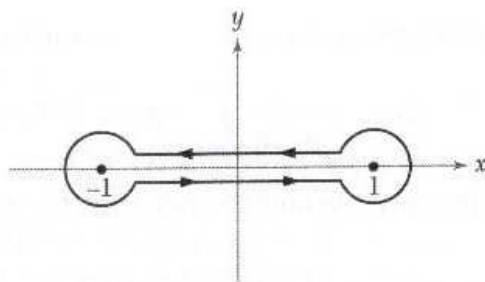
Figure 4.3.11: Contour for evaluating \int_0^1 \frac{dx}{\sqrt{x^2-1}} .
