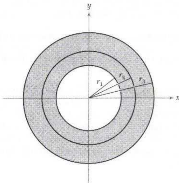
Figure 2.5.4: Hadamard's Three-circle Theorem.
