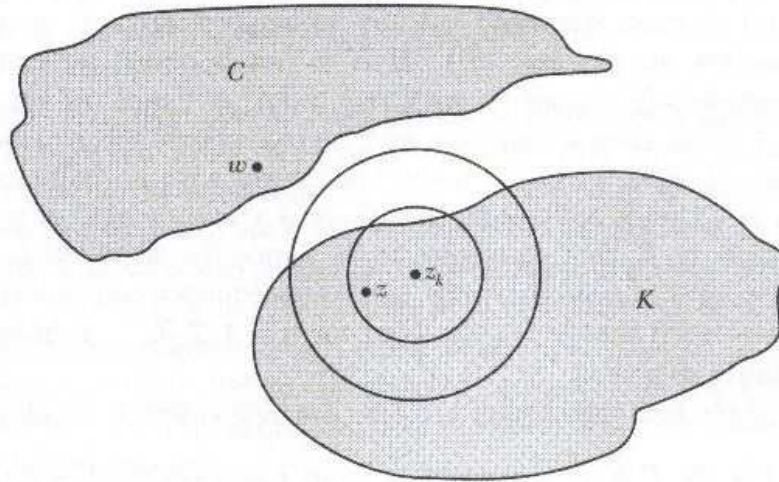
Figure 1.4.6: The distance between a closed set C and a compact set K is greater than zero.
