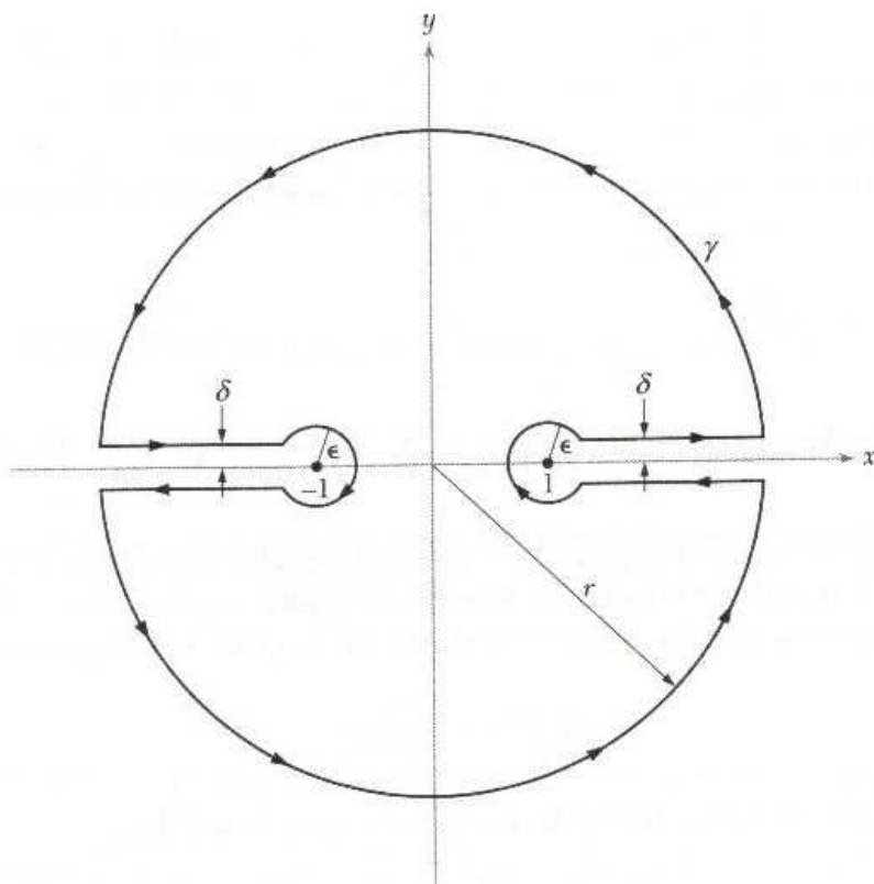
Figure 4.3.8: The curve \gamma used for Worked Example 4.3.21.
