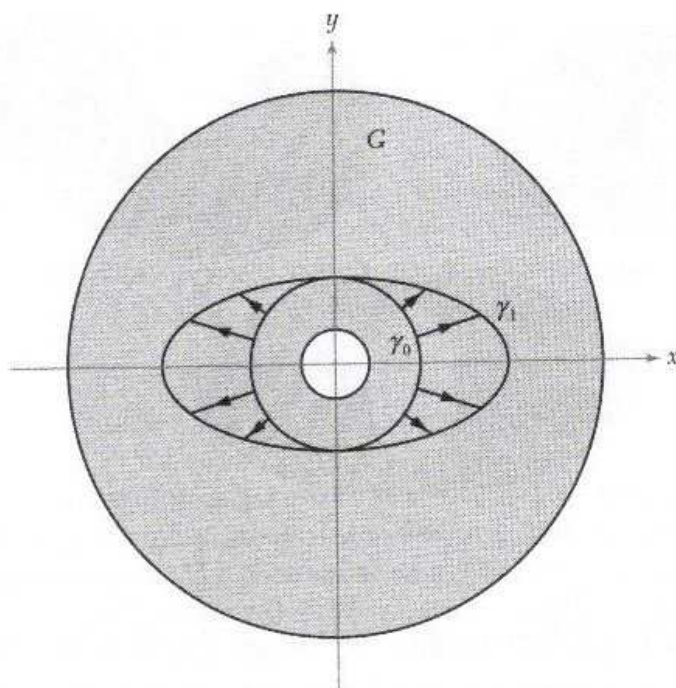
Figure 2.3.10: A circle homotopic to an ellipse.
