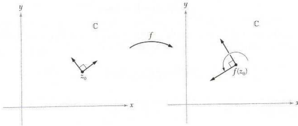
Figure 1.5.1: Conformal at z_0 .
