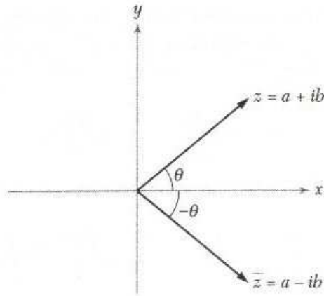
Figure 1.2.8: Complex conjugation.
