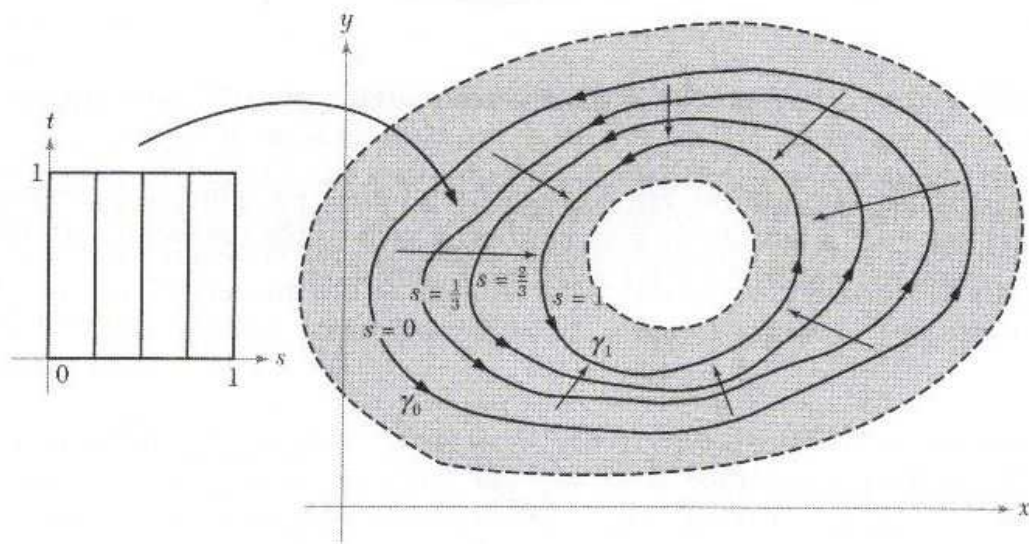
Figure 2.3.9: Closed-curve homotopy.
