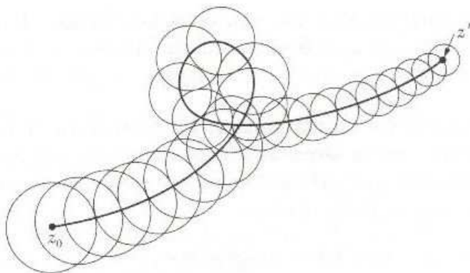
Figure 6.1.8: Continuation can lead to self-intersections.
