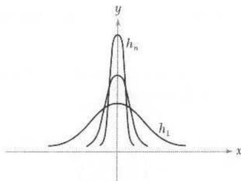
Figure 7.2.4: Approximating \delta sequence.
