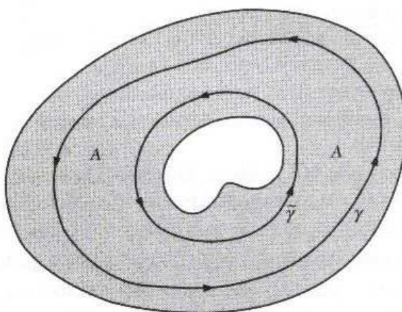
Figure 2.2.3: Deformation theorem.
