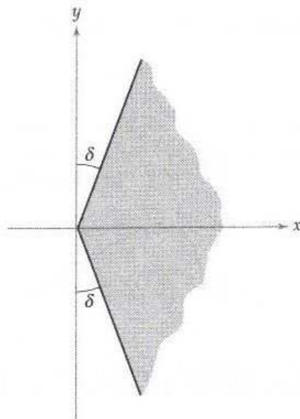
Figure 7.3.1: Region of validity for Stirling's formula.
