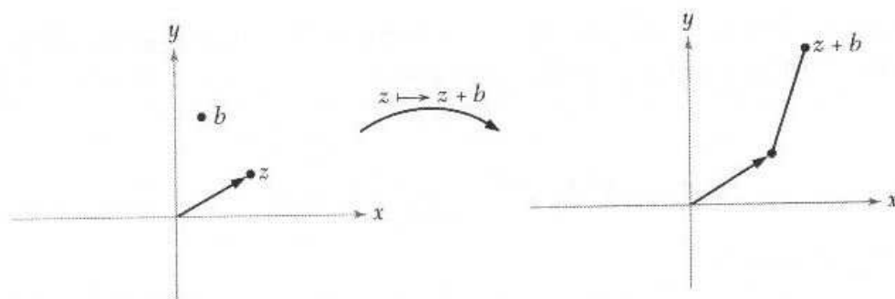
Figure 5.2.1: Translation.
