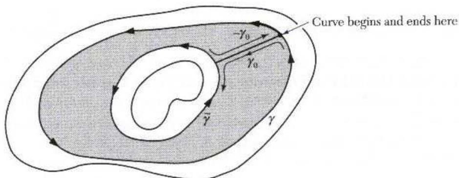
Figure 2.2.4: Curve used to prove the Deformation Theorem.
