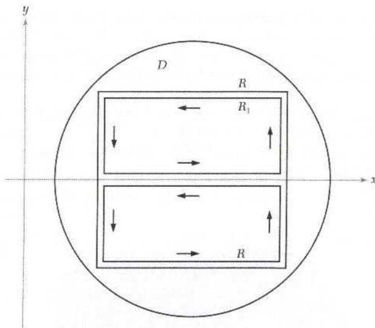
Figure 2.4.7: Construction used to show \int_R f = 0 .
