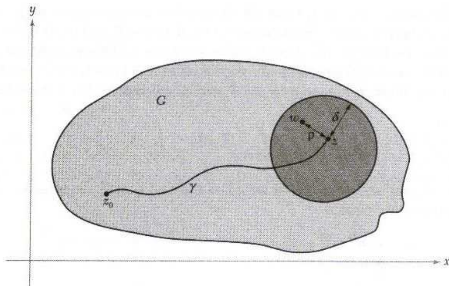
Figure 2.1.7: Defining an antiderivative by an integral.
