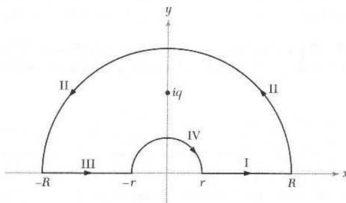
Figure 4.3.6: Contour used for Example 4.3.18.
