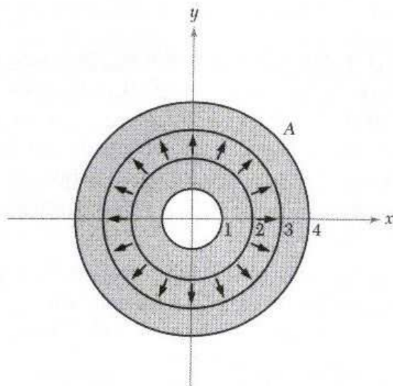
Figure 2.3.17: Region that is not simply connected.
