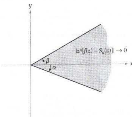
Figure 7.2.1: Asymptotic expansion.
