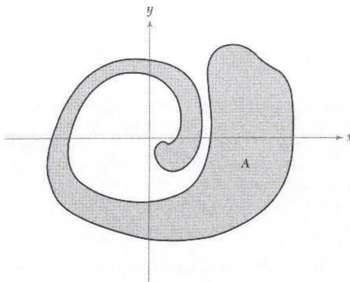
Figure 2.2.7: A possible domain for the log function.
