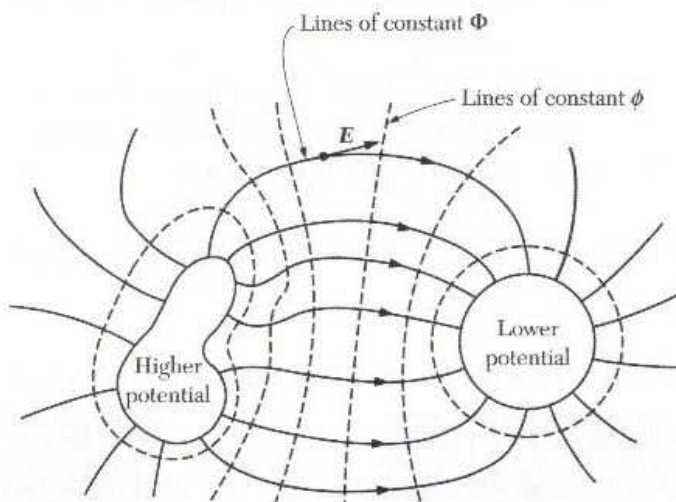
Figure 5.3.8: Electrical potential.
