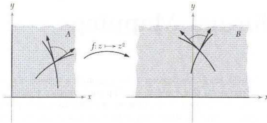
Figure 5.1.1: A conformal map.
