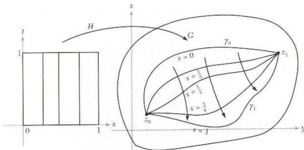
Figure 2.3.7: Fixed-endpoint homotopy.
