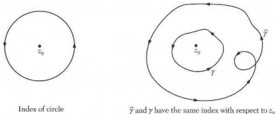
Figure 2.4.2: Index = the number of times that z_0 is encircled.
