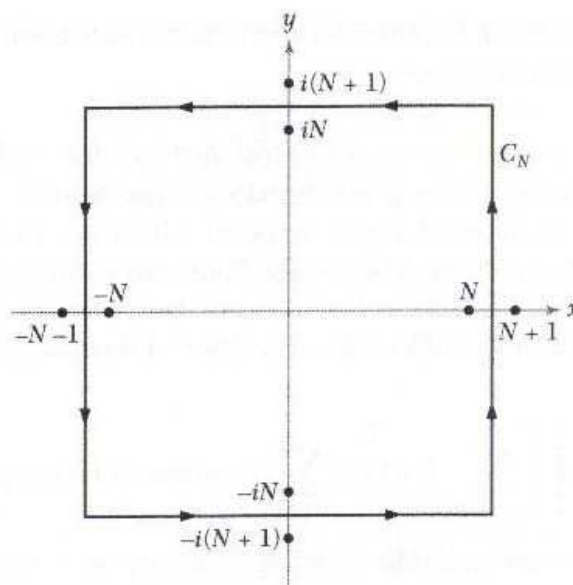
Figure 4.4.1: Contour for evaluating \sum_{-\infty}^{\infty} f(n) .
