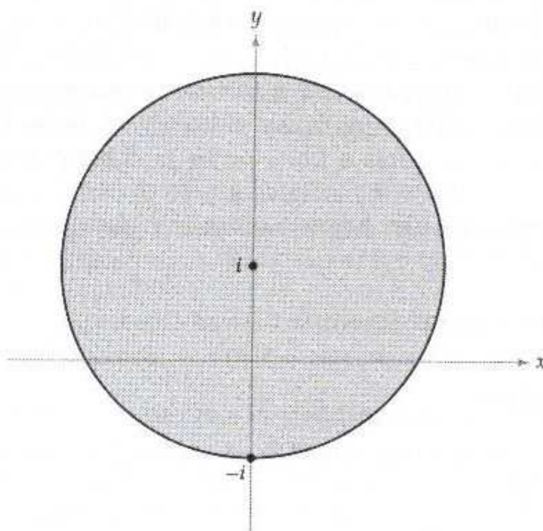
Figure 3.3.4: Region of convergence for the expansion of 1/(z+i) .
