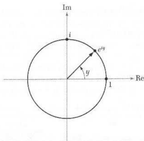
Figure 1.3.1: Points on the unit circle.
