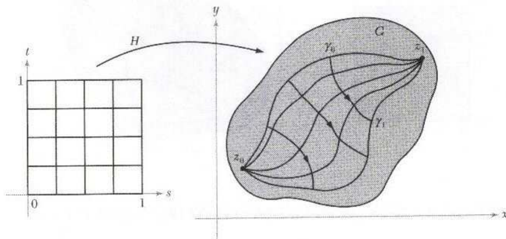
Figure 2.3.12: Fixed-endpoint homotopy.
