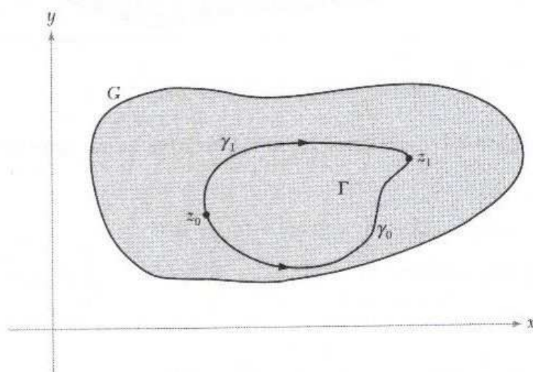
Figure 2.1.6: \gamma_0 - \gamma_1 = \Gamma .
