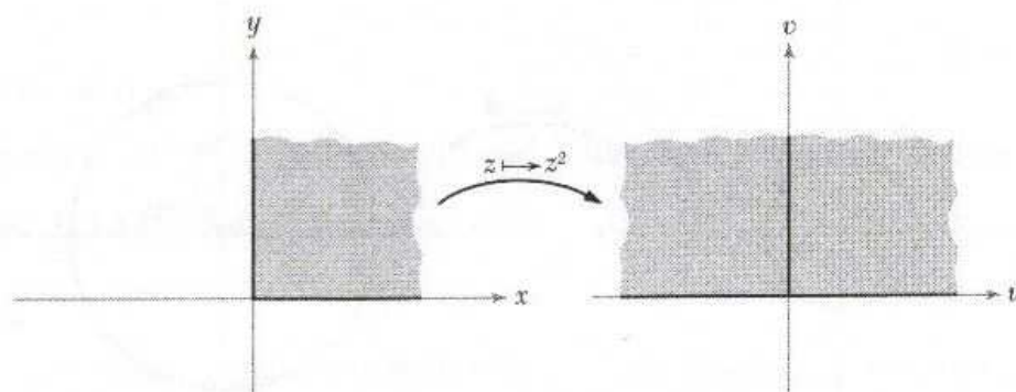
Figure 1.3.3: Squaring function.
