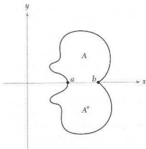
Figure 6.1.5: A^* is the reflection of A .
