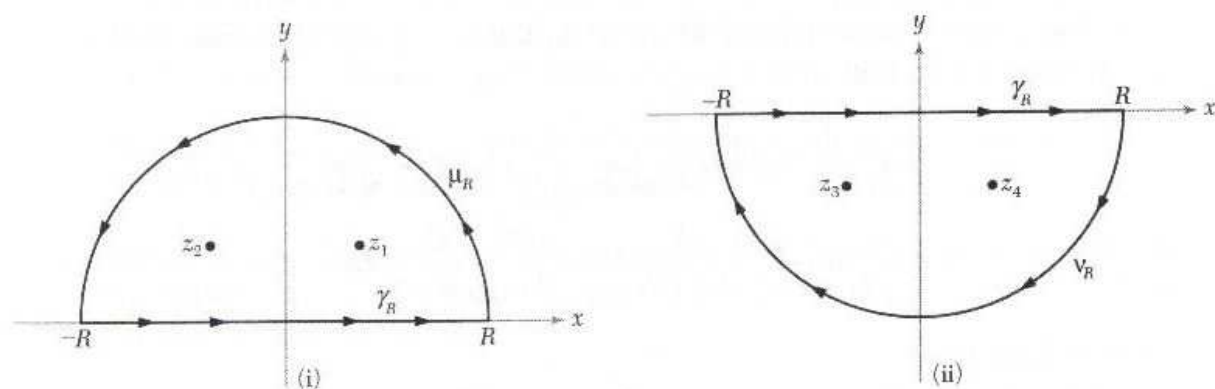
Figure 4.3.1: Curves for two solutions to Example 4.3.5
