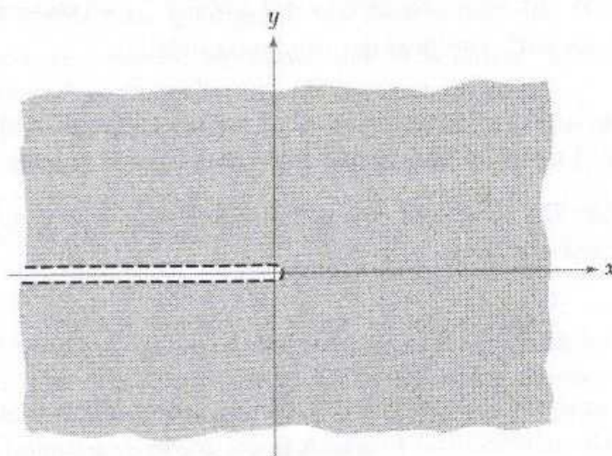
Figure 1.6.1: Domain of \log z .
