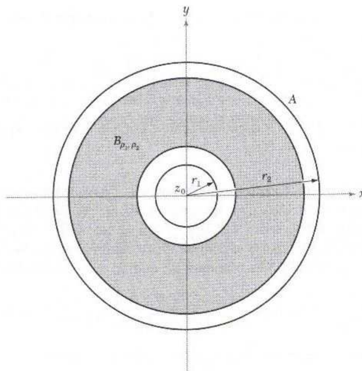
Figure 3.3.1: Laurent series, with z_0 = 0 .
