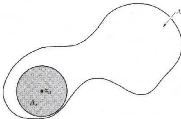
Figure 3.2.2: Taylor's Theorem.
