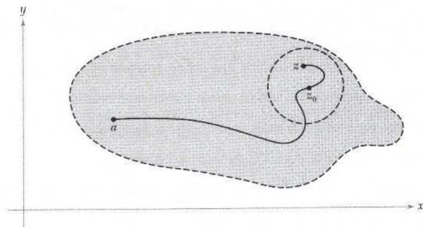
Figure 1.4.5: An open connected set is path-connected.
