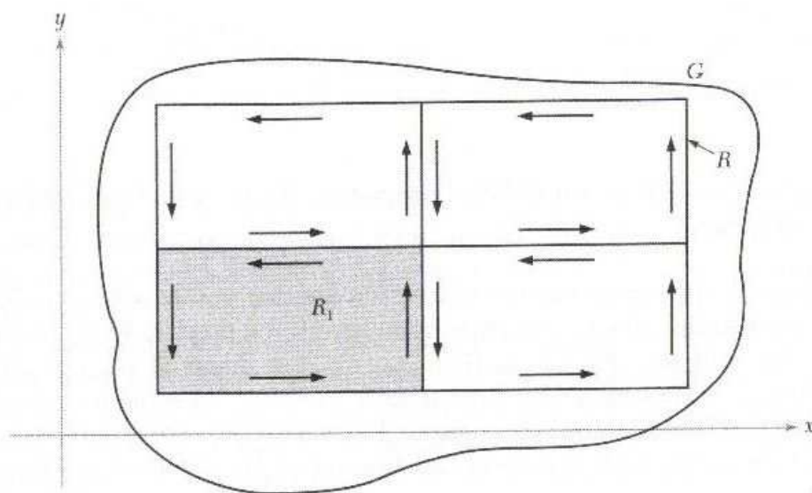
Figure 2.3.1: Bisection procedure.
