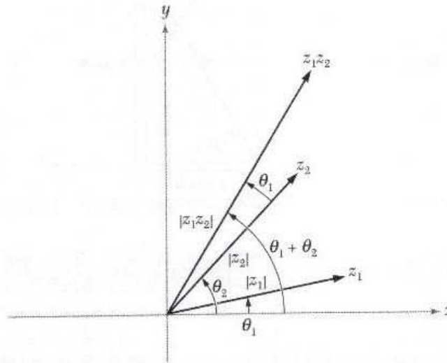
Figure 1.2.4: Multiplication of complex numbers.
