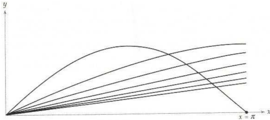
Figure 3.1.7: y = \sin(x/n) for n = 1 through 7.
