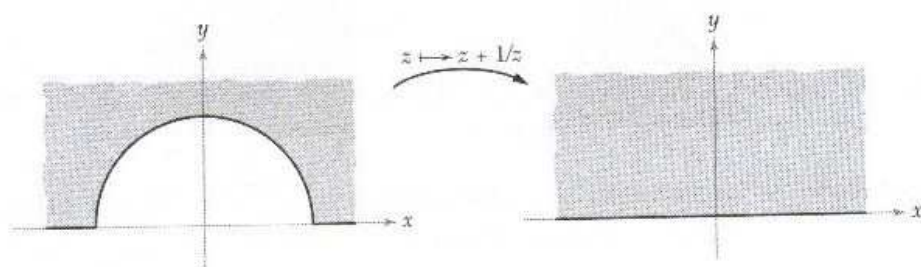
Figure 5.3.16: Effect of z \mapsto z + 1/z .
