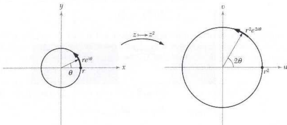
Figure 1.3.5: Squaring function and its inverse.
