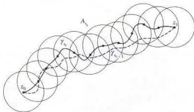
Figure 6.1.12: Each \gamma_{s_{k+1}} is contained in A_{s_k} .
