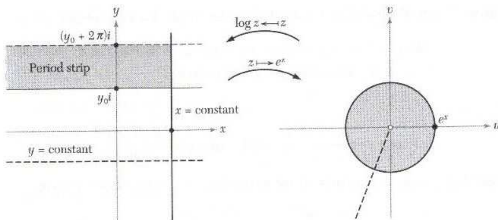
Figure 1.3.7: Geometry of e^z and \log z .
