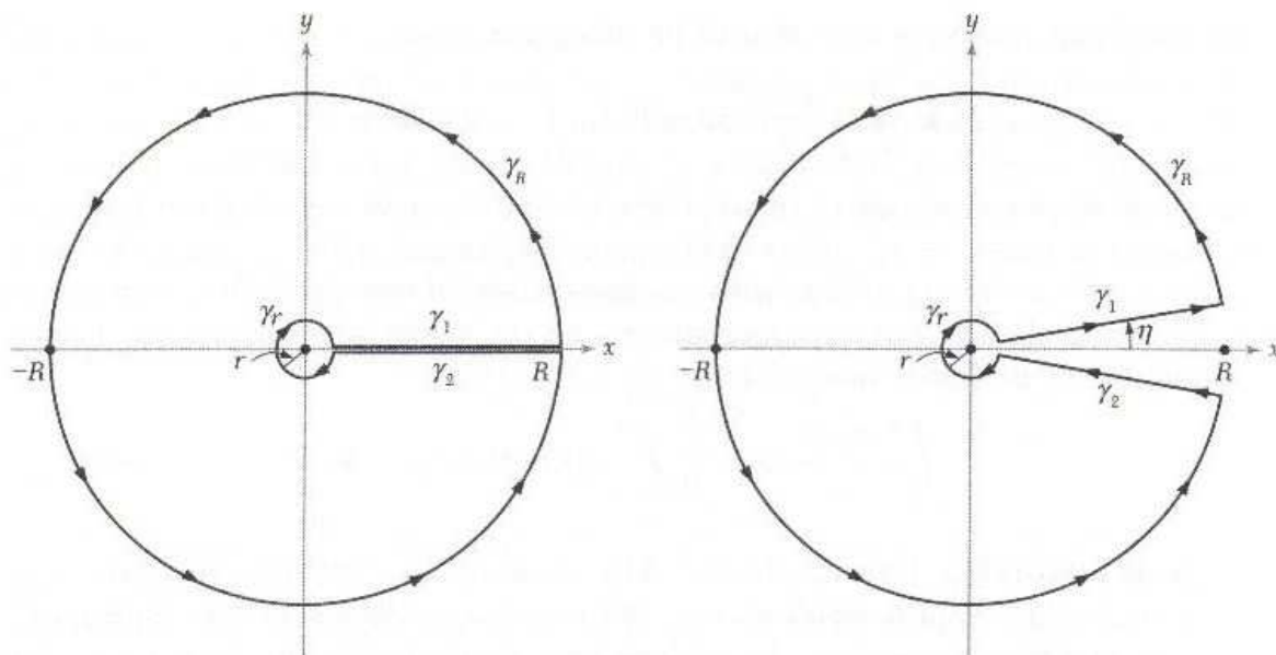
Figure 4.3.5: Contours for the Mellin transform integral.
