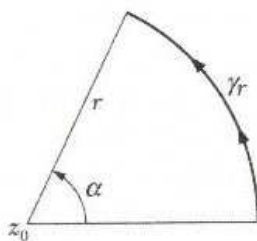
Figure 4.3.4: Integrate part way around a simple pole.
