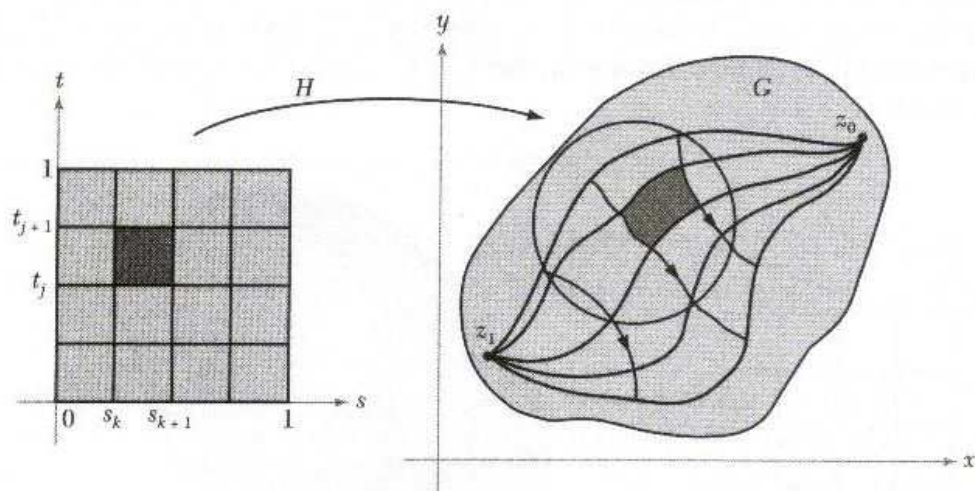
Figure 2.3.14: Subdivision for proof of the Deformation Theorem.
