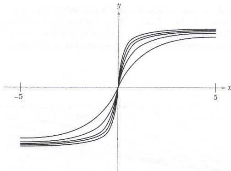
Figure 3.1.8: y = \arctan(nx) for n = 1 through 5.
