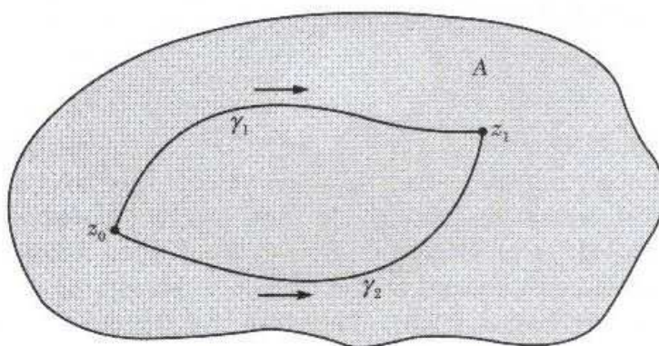
Figure 2.2.6: Independence of path.
