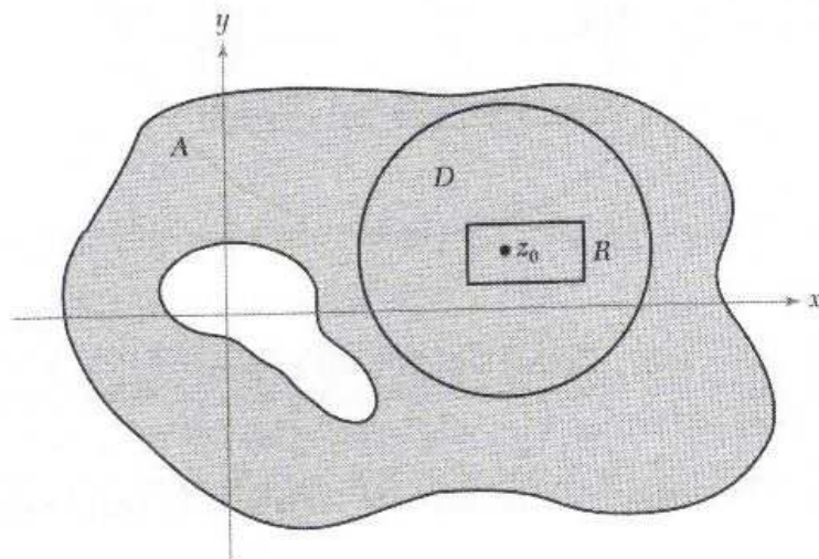
Figure 2.4.6: If \int_R f = 0 , then f is analytic.
