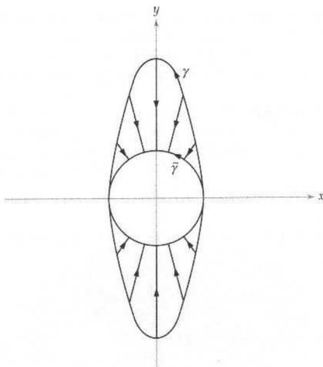
Figure 2.4.5: Homotopy of \gamma(t) = (\cos t, 3\sin t) to \tilde{\gamma}(t) = (\cos t, \sin t) .
