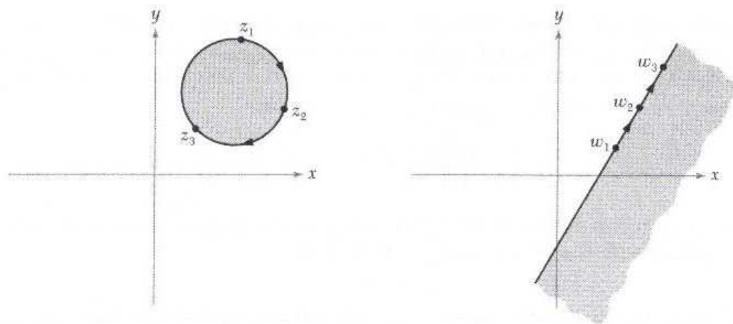
Figure 5.2.3: Effect of a fractional linear transformation.
