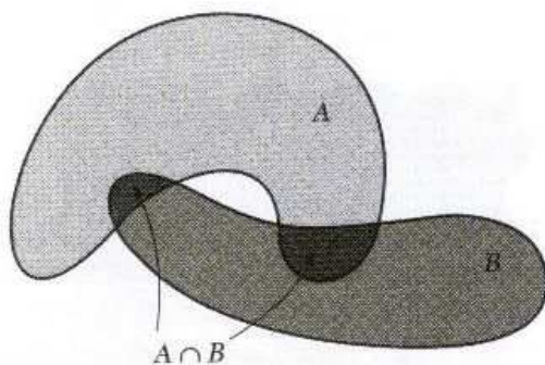
Figure 6.1.2: Analytic continuation.
