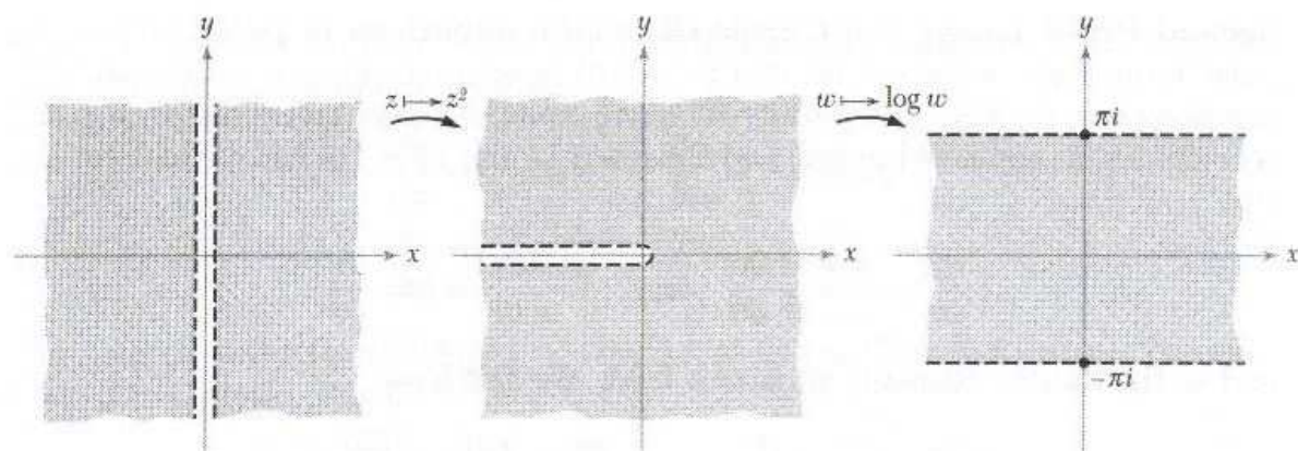
Figure 1.6.2: Composing the squaring and the log functions.
