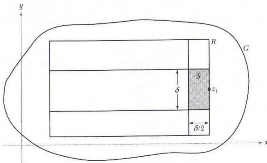
Figure 2.3.6: What happens if z_1 lies on R .
