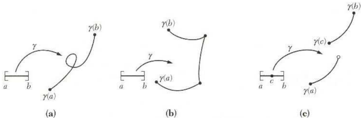
Figure 2.1.1: Curves in the complex plane \mathbb{C} . (a) Smooth curve. (b) Piecewise C^1 curve. (c) Discontinuous curve.
