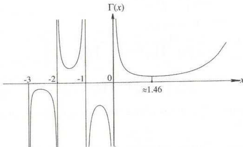
Figure 7.1.1: The graph of \Gamma(x) for x real.
