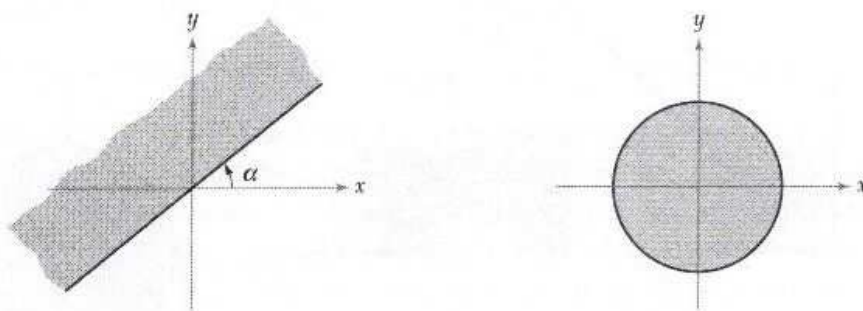
Figure 5.2.8: Mapping a rotated half plane to the disk.
