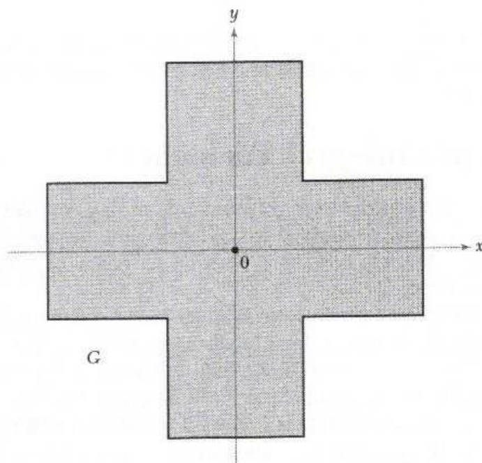
Figure 2.3.18: A star-shaped nonconvex region.
