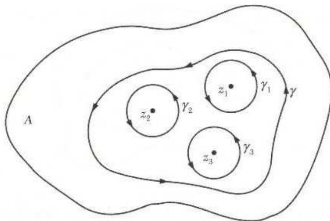
Figure 4.2.2: First intuitive proof of the Residue Theorem.
