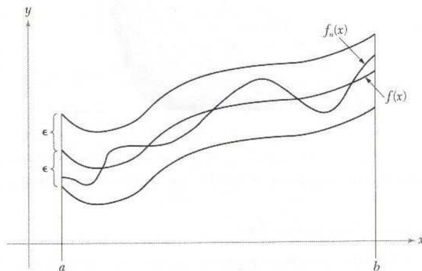
Figure 3.1.1: Uniform convergence on an interval [a, b] .
