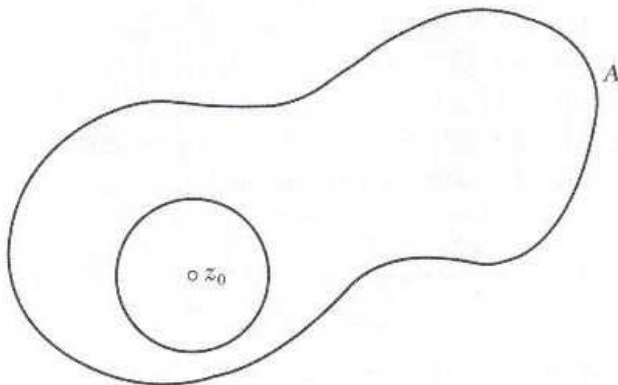
Figure 3.3.3: Isolated singularity.
