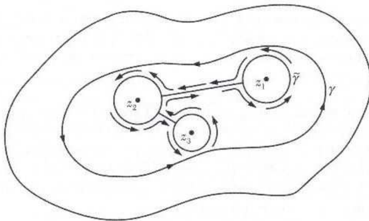
Figure 4.2.3: Second intuitive proof of the Residue Theorem.
