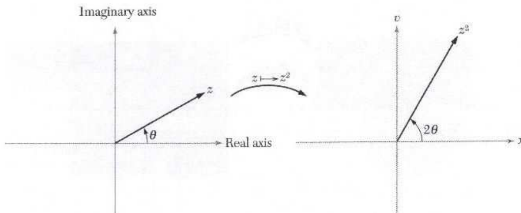
Figure 1.3.3: Squaring function.
