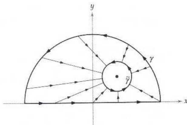
Figure 4.2.8: Homotopy between \gamma and \tilde{\gamma} .
