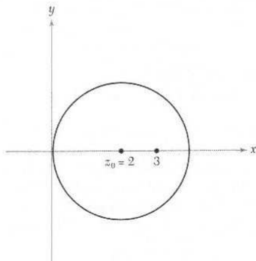
Figure 3.2.3: The circle of convergence for the power series in Worked Example 3.2.12 must be at least this big.
