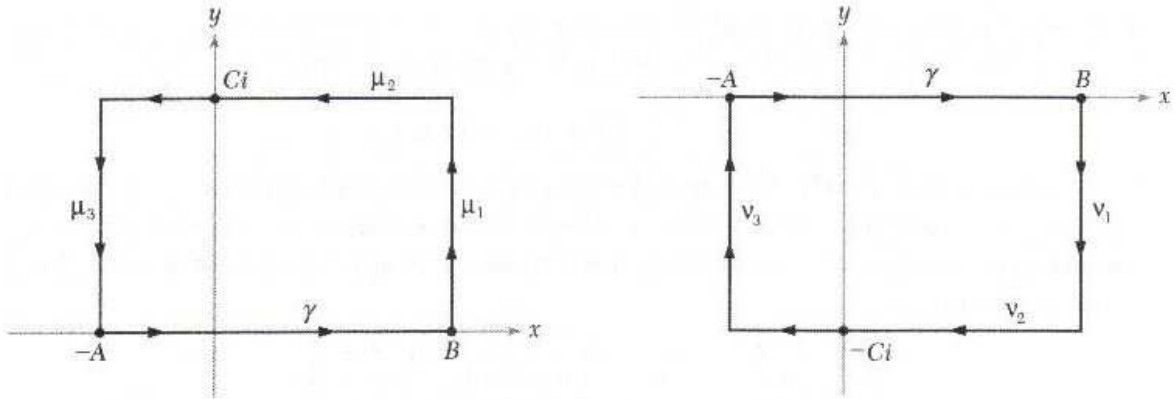
Figure 4.3.2: Paths for Example 4.3.8.
