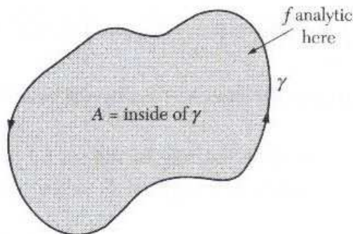
Figure 2.2.1: Cauchy's Theorem: \int_{\gamma} f = 0 .
