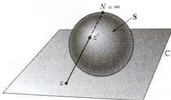
Figure 1.4.8: Riemann sphere.
