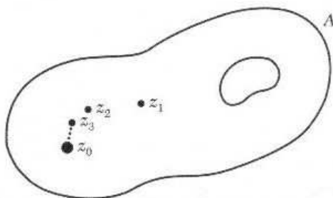
Figure 6.1.1: Identity Theorem: If f = g at all the points z_1, z_2, \dots , then f(z) = g(z) for all z \in A .
