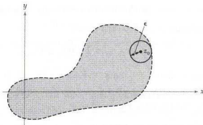
Figure 1.4.1: Open set.
