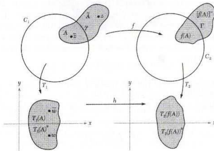
Figure 6.1.6: Analytic continuation by reflection.
