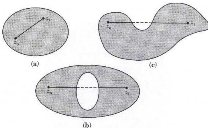
Figure 2.3.11: (a) Convex set. (b) and (c) Sets that are not convex.
