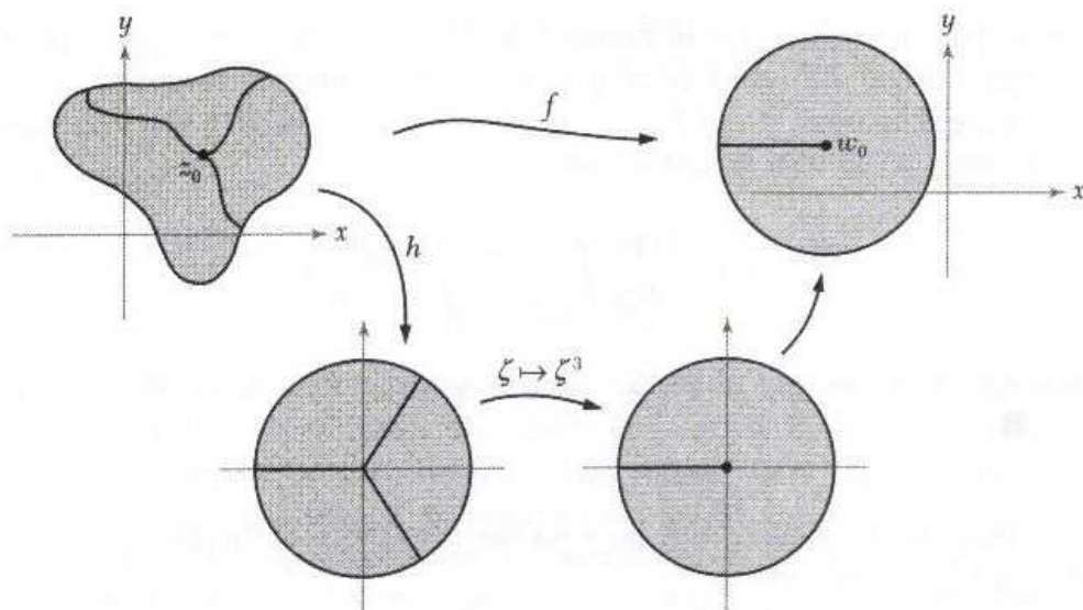
Figure 6.3.2: Worked Example 6.3.6 with k = 3 .
