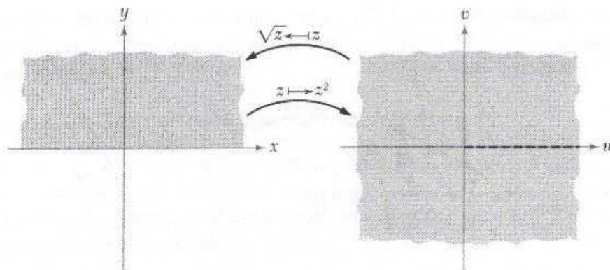
Figure 1.3.5: Squaring function and its inverse.
