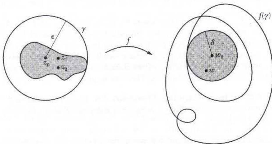
Figure 6.3.1: This function is two-to-one near z_0 .
