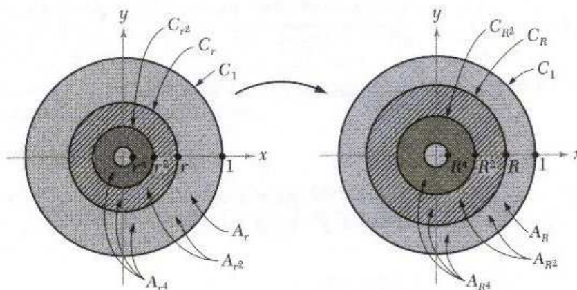
Figure 6.1.20: Conformal maps of annuli.
