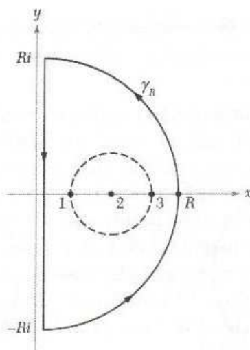
Figure 6.2.7: Contour for Exercise 3.
