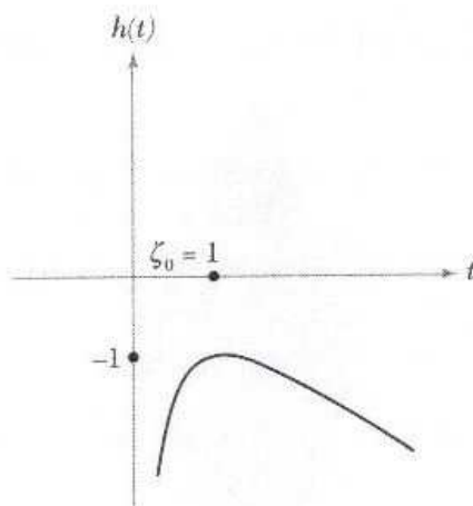
Figure 7.3.2: Graph of h(t) = \log t - t .
