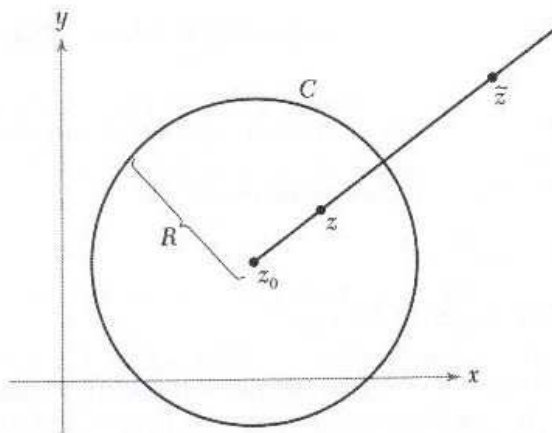
Figure 5.2.5: Reflection of z in C .
