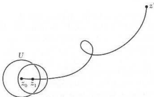
Figure 6.1.7: Continuation by power series.
