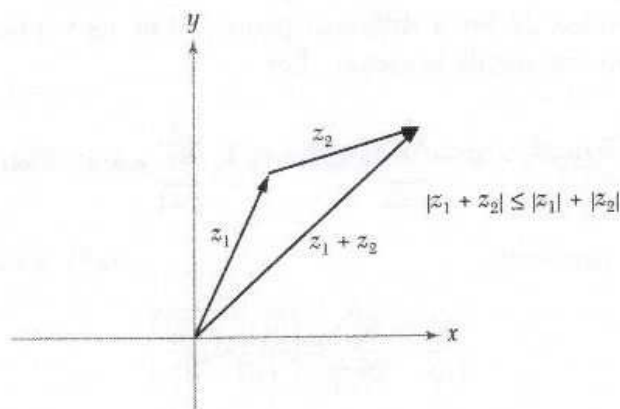
Figure 1.2.9: Triangle inequality.
