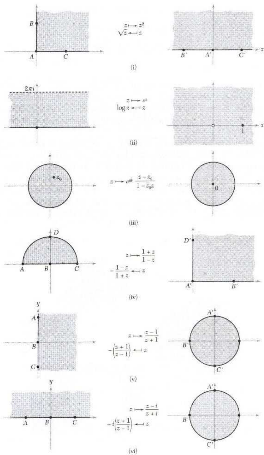
Figure 5.2.10: Some common transformations.
