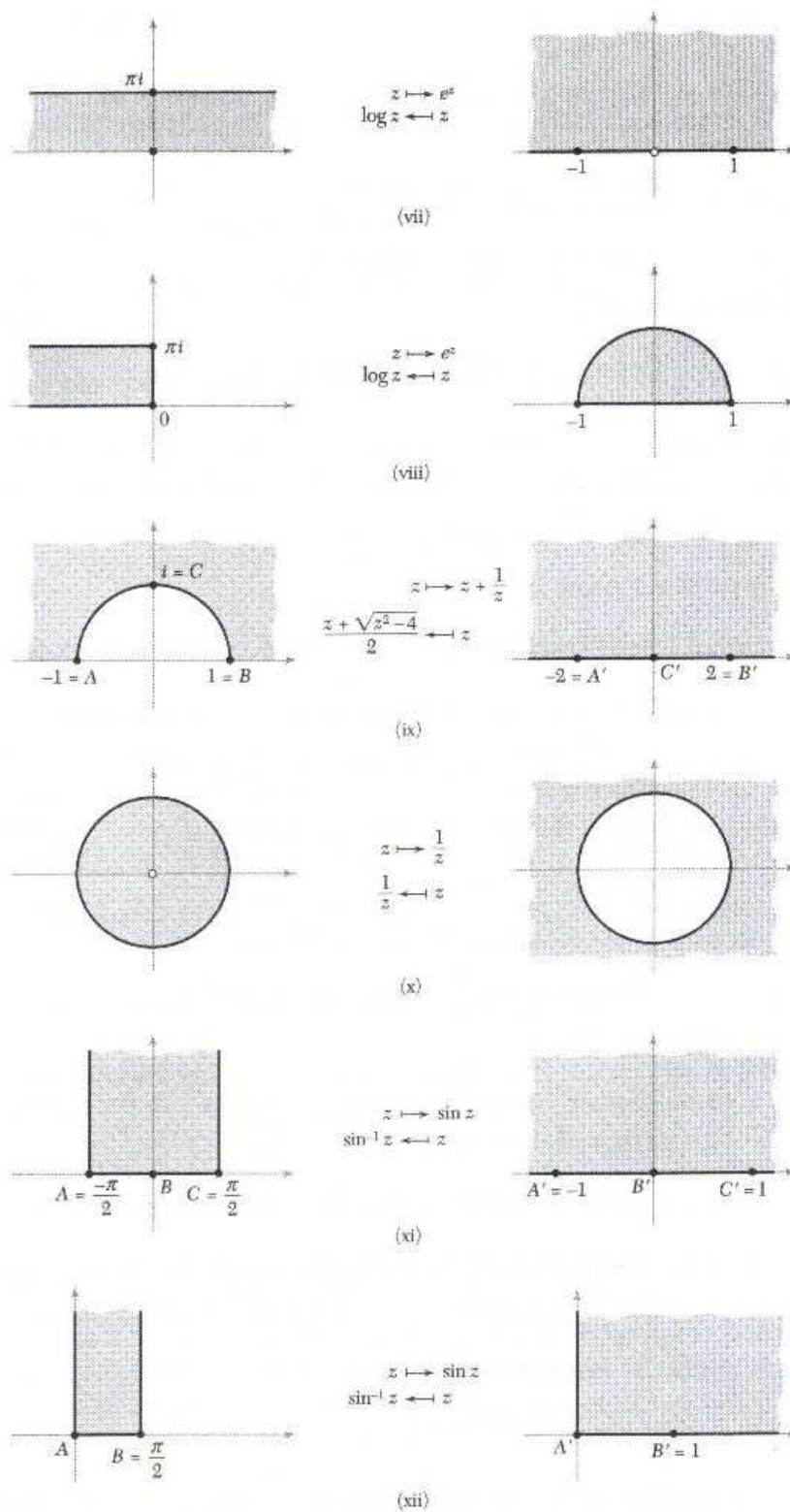
Figure 5.2.11: More common transformations.
