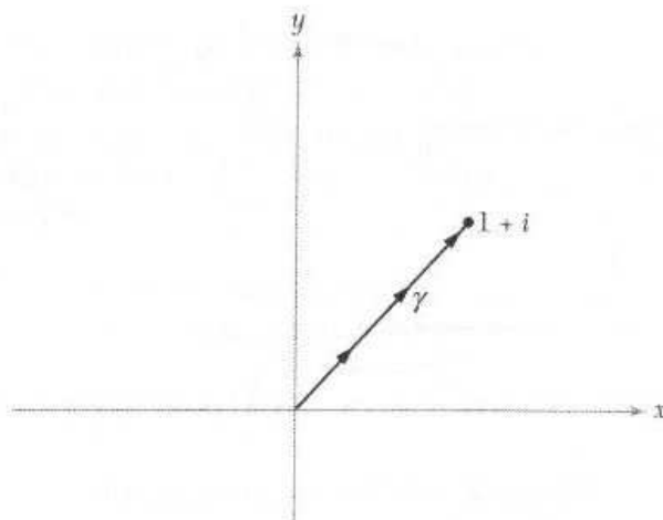
Figure 2.1.5: Curve from 0 to 1 + i .
