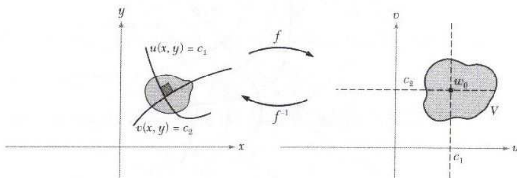
Figure 1.5.6: Since f and f^{-1} are analytic, they are conformal and so preserve orthogonality.
