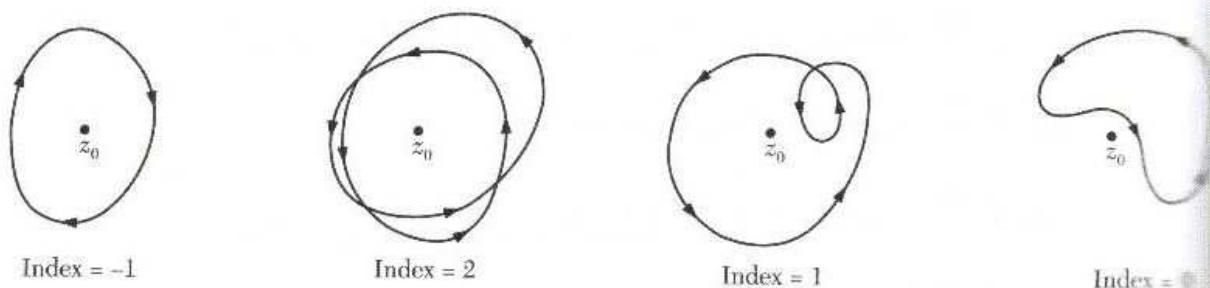
Figure 2.4.1: Index of a curve around a point.
