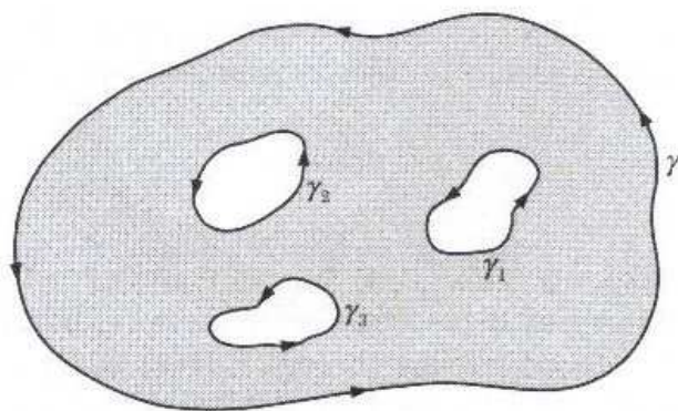
Figure 2.2.9: Generalized Deformation Theorem.
