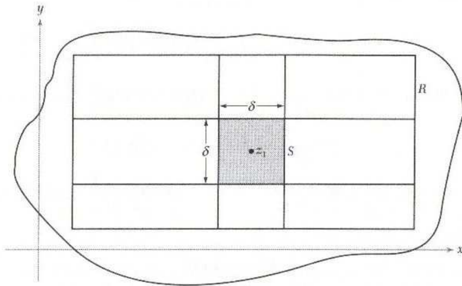
Figure 2.3.5: Construction of S and subdivision of R for the proof of Lemma 2.3.3.
