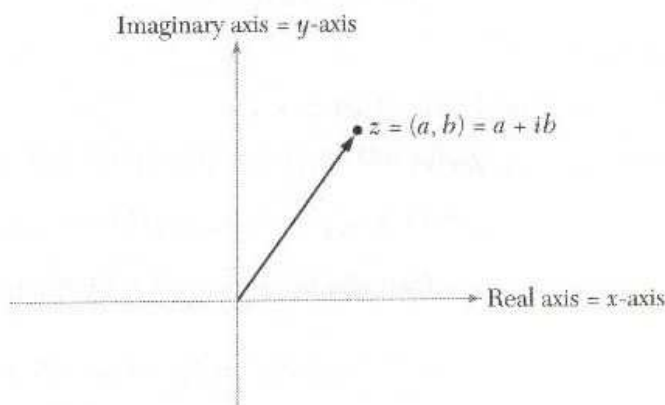
Figure 1.2.1: Vector representation of complex numbers.
