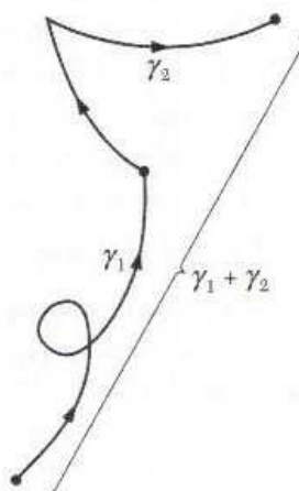
Figure 2.1.3: Join of two curves.
