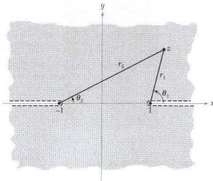
Figure 1.6.5: Domain of analyticity of \sqrt{z^2 - 1} .
