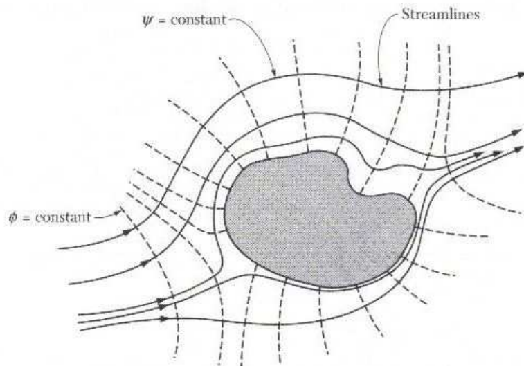
Figure 5.3.14: Fluid flow.
