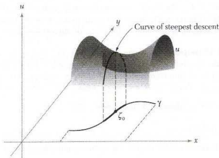
Figure 7.2.2: Saddle-point method.
