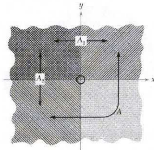
Figure 6.1.4: Continuing the log.
