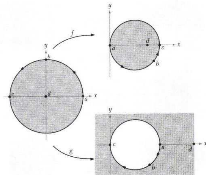
Figure 5.2.9: The maps for Worked Example 5.2.15.
