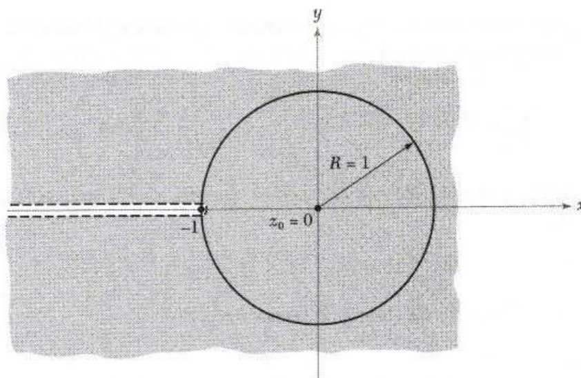
Figure 3.2.4: Taylor series of \log(1+z) .
