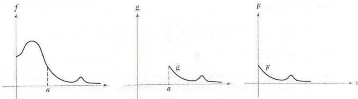
Figure 8.1.3: F is obtained from f by shifting and truncating.
