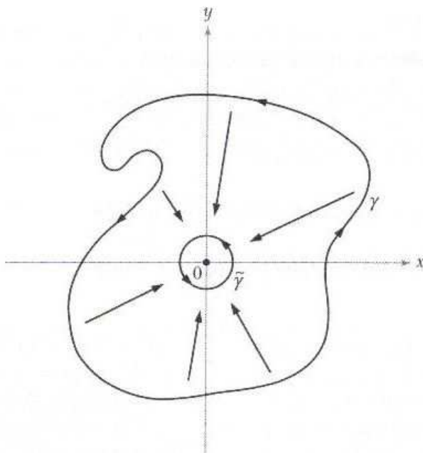
Figure 2.2.8: Deformation of \gamma to the circle \tilde{\gamma} .
