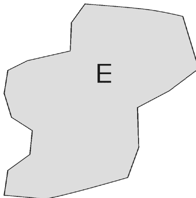
Figure 3.1: A compact set.
